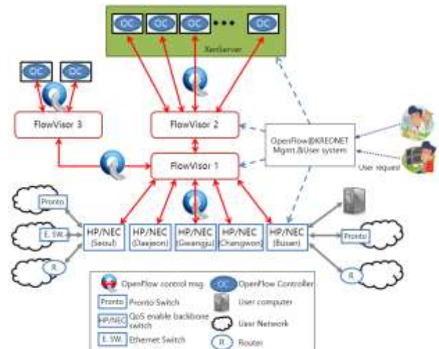
Figure 2. OpenFlow@KREONET
