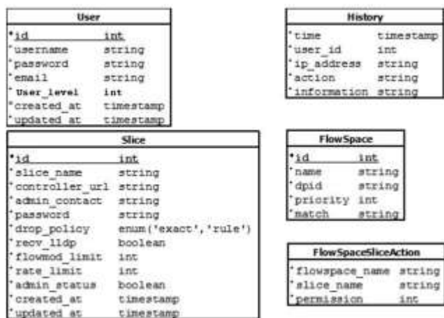
Figure 6. DB schema
