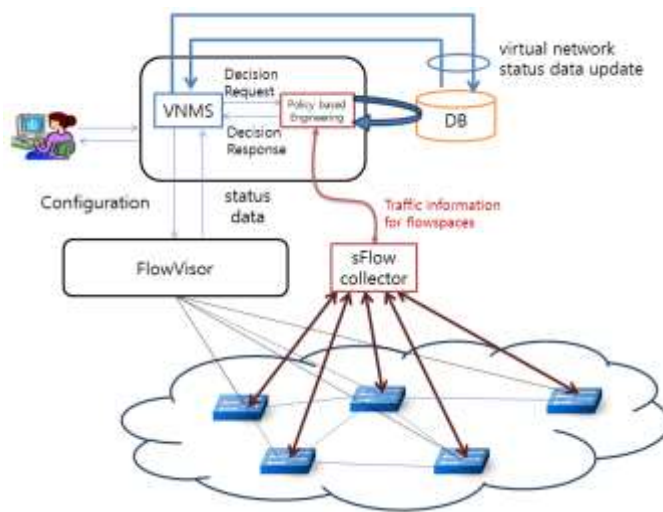
Figure 4. the Policy based Engineering module in OF@KREONET Virtual Network Management System
